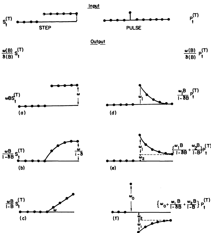
a (a), (b), (c) show the response to a step input for various simple transfer function models; (d), (e), (f) show the response to a pulse for some models of interest.
